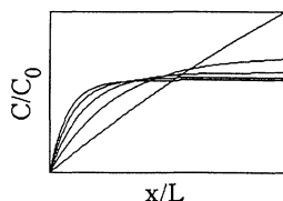
FIG. 2. The concentration of anions in the cell, as a function of the fluid speed, for typical values of the concentration and the applied voltage. When there is no fluid flow, the concentration varies linearly in the cell, as in Chazalviel's model (without convection). When the fluid flow is incorporated in the model, the shape of the concentration is no longer linear. Also, the size of the space charge (which is very small with the value C = 10^{18} taken here) decreases when v increases.
