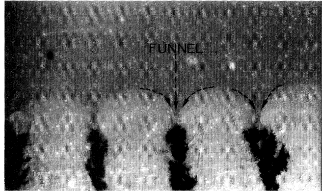
FIG. 6. Experimental observation of the fluid motion, in typical conditions (cell dimensions 1 \text{ cm} \times 1 \text{ cm} \times 0.1 \text{ mm} , copper sulphate, concentration 5 \times 10^{-2} \text{ mol l}^{-1} , voltage 5 \text{ V} ). The fluid motion is made visible by means of small droplets of oil (hence the rough aspect of the picture). The oil droplets are trapped in the deposit and do not penetrate inside the vortices, hence the upper part of the picture appears darker than the inner part of the vortices; this allows us to see the funnel which is formed on top of the contrarotative vortices, which are found on each side of a tip. The concentration of copper sulphate is almost constant in this funnel. The space charge is found at the foot of the arch, in a very narrow region, which probably encompasses a small part of the branch. The fluid flow, which is always inwards at the tips, reduces the size of the space charge by a factor \approx 1.2(E_{\text{bulk}}/v)^{1/3} , where v is the speed at the tip.
