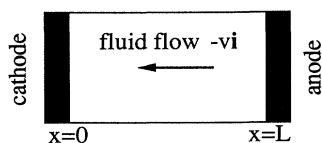
FIG. 1. Scheme of the cell for the model discussed in Sec. II. The fluid flow is a constant flow going from the anode towards the cathode. The fluid flow is supposed not to bring ions in at the anode nor to take the ions away behind the cathode.
