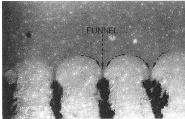
FIG. 6. Experimental observation of the fluid motion, in typical conditions (cell dimensions 1\text{ cm} \times 1\text{ cm} \times 0.1\text{ mm} , copper sulphate, concentration 5 \times 10^{-2}\text{ mol l}^{-1} , voltage 5\text{ V} ). The fluid motion is made visible by means of small droplets of oil (hence the rough aspect of the picture). The oil droplets are trapped in the deposit and do not penetrate inside the vortices, hence the upper part of the picture appears darker than the inner part of the vortices; this allows us to see the funnel which is formed on top of the contrarotative vortices, which are found on each side of a tip. The concentration of copper sulphate is almost constant in this funnel. The space charge is found at the foot of the arch, in a very narrow region, which probably encompasses a small part of the branch. The fluid flow, which is always inwards at the tips, reduces the size of the space charge by a factor \approx 1.2(E_{\text{bulk}}/v)^{1/3} , where v is the speed at the tip.
