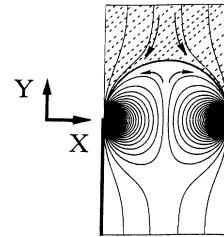
FIG. 5. The fluid stream between two neighboring tips, in the moving frame which advances with the anions. The arrows show the fluid motion. This shape compares rather well with the observed one, except in the zone of the tip, where this theoretical stream is singular, while the real stream, of course, is not. The dashed area is the concentrated area, where the concentration is almost constant, and equal to the bulk concentration. Inside the vortices, the concentration is almost equal to zero. Hence the cations go towards the tip through some kind of a funnel which lies above the vortices (the dashed zone).
