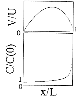
FIG. 3. The potential and the concentration of cations across the cell, in the case of a very fast fluid flow ( v=0.4 \text{ cm s}^{-1} ). In this instance, the concentration must be taken as infinite near the anode, because the dissolution of the anode is, in theory, instantaneous.
